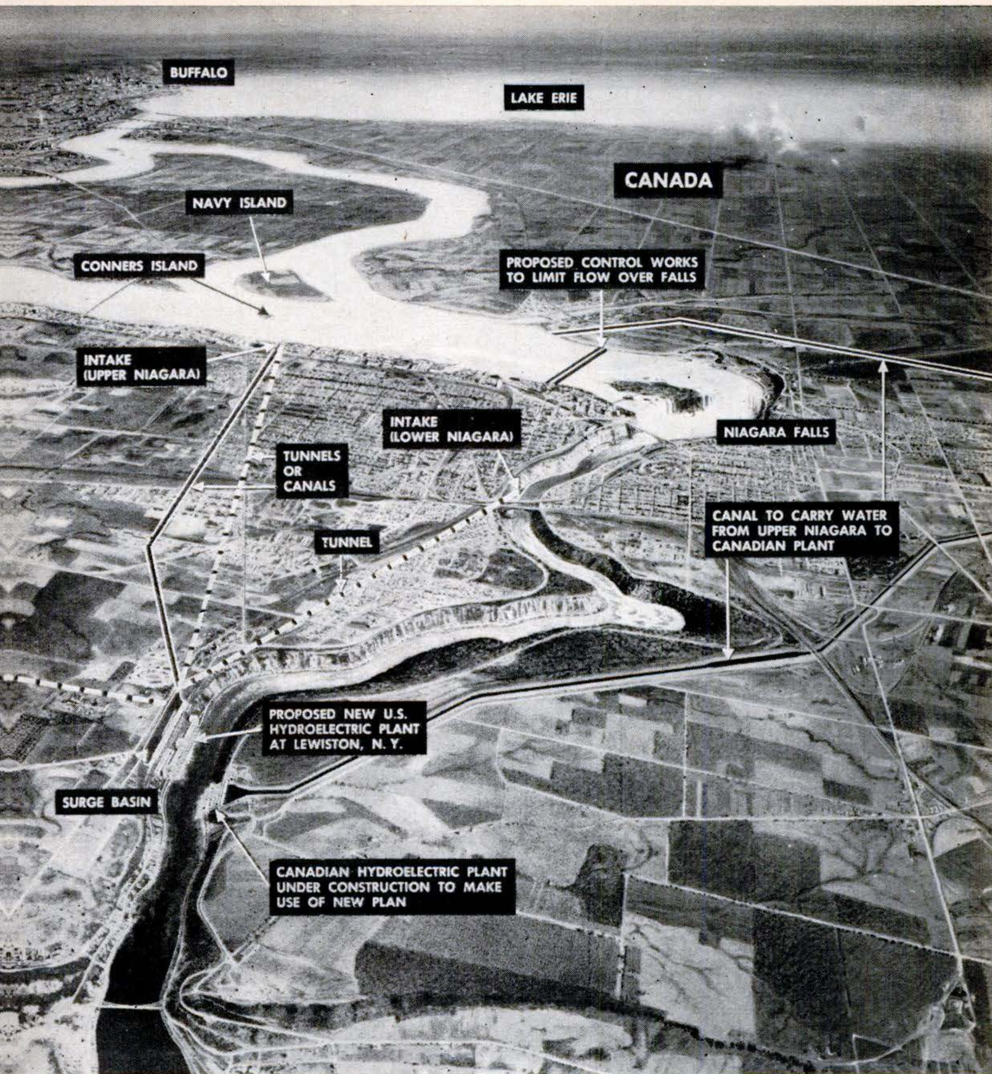
States and Canada will tap the Niagara River to get more electricity for both nations.
